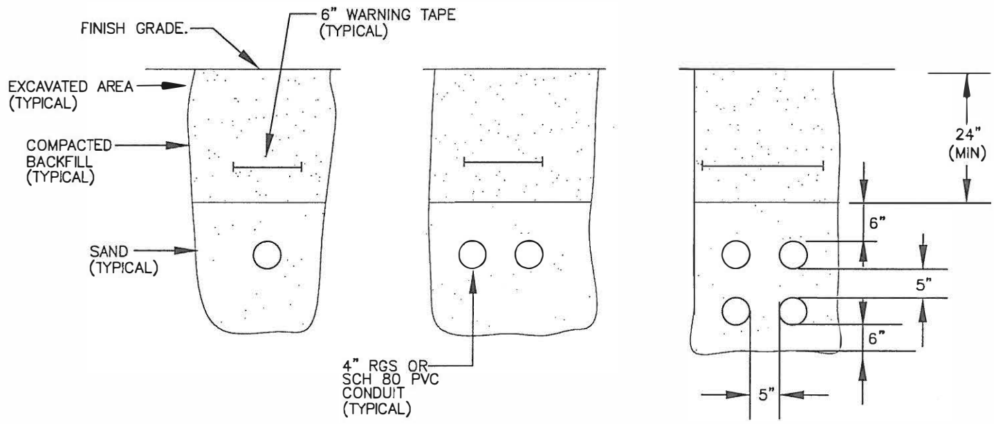
SHALLOW INSTALLATION WITH RGS OR SCH 80 PVC CONDUIT IN SAND
